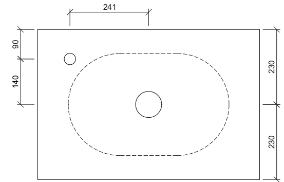
Taphole Offset
