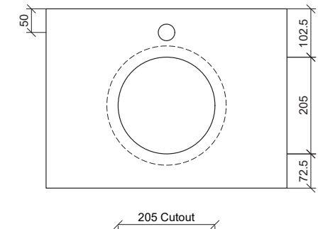
Taphole Behind
