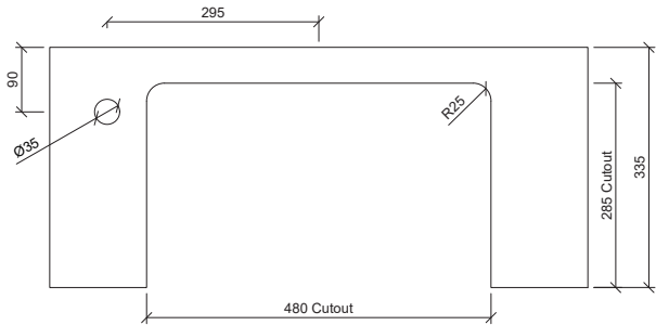
Taphole Offset
