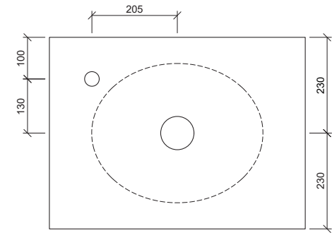
Taphole Offset
