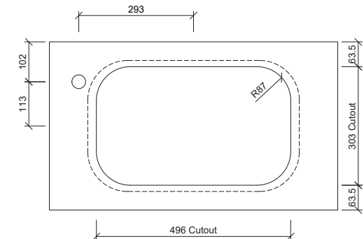
Taphole Offset
