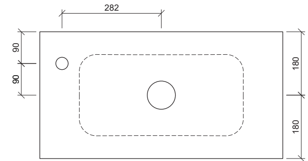
Taphole Offset
