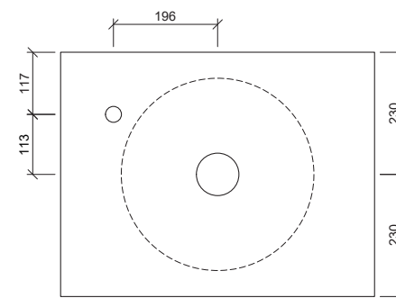
Taphole Offset
