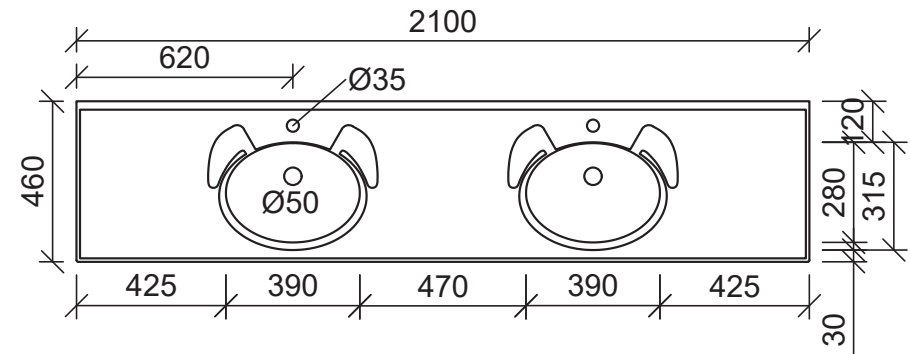
Top View
