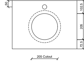
Taphole Behind
