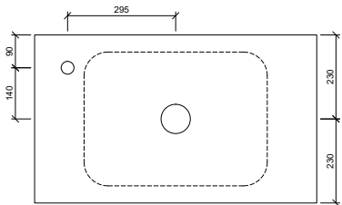
Taphole Offset
