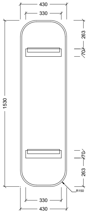
BACKING BOARD
