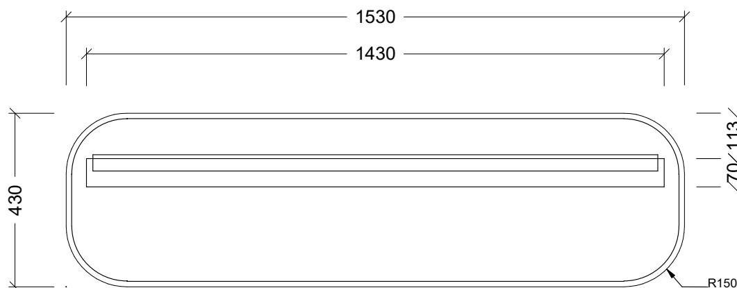
BACKING BOARD
