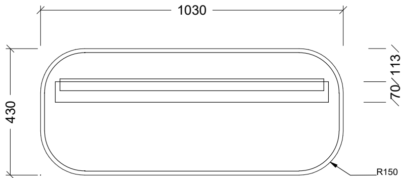
BACKING BOARD
