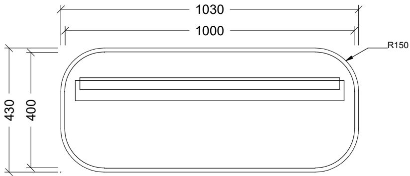
MIRROR
