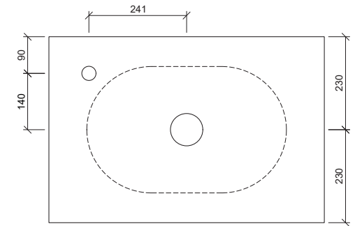
Taphole Offset
