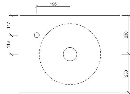
Taphole Offset
