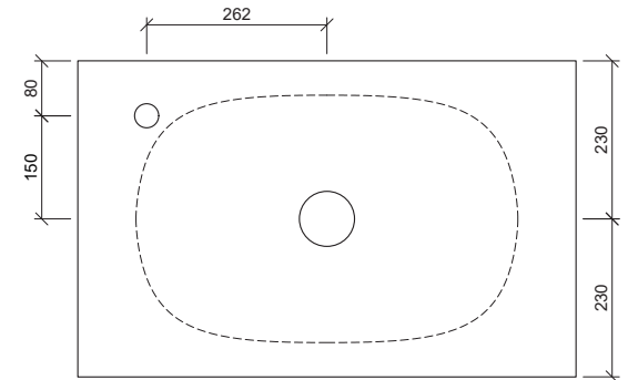
Taphole Offset
