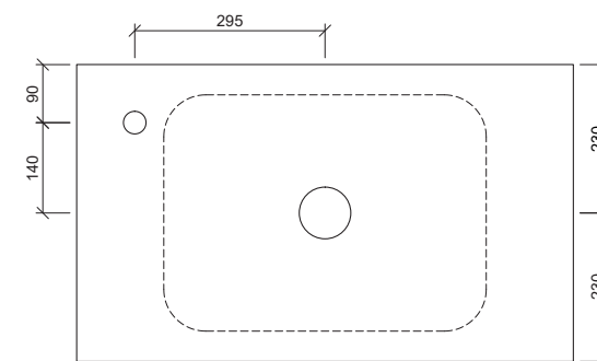
Taphole Offset
