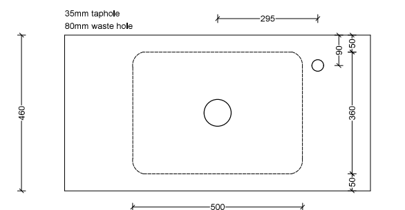
Taphole Offset
